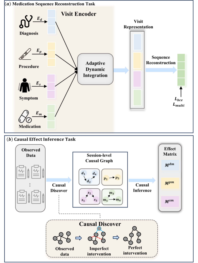
Fig. 3. Pretraining Framework. (a) Medication Sequence Reconstruction task. (b) Causal Effect Inference task.
