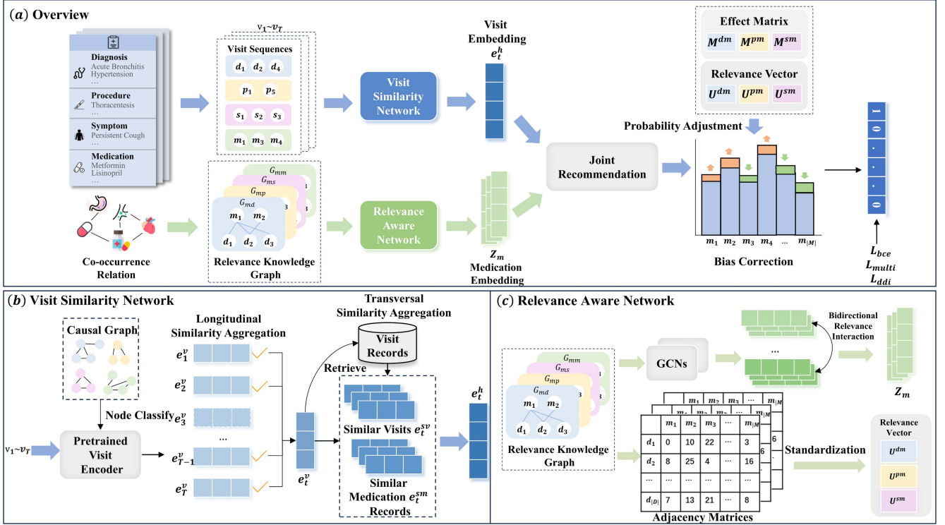
Fig. 2. (a) Overview of RaVSNet (b) Visit Similarity Network, which generates the visit representation using the similarity information; (c) Relevance Aware Network, which is used to mine the internal relevance knowledge in the medical information.
