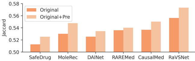
Fig. 5. Accuracy comparison of baselines and their variants with pre-training framework of RaVSNet.
