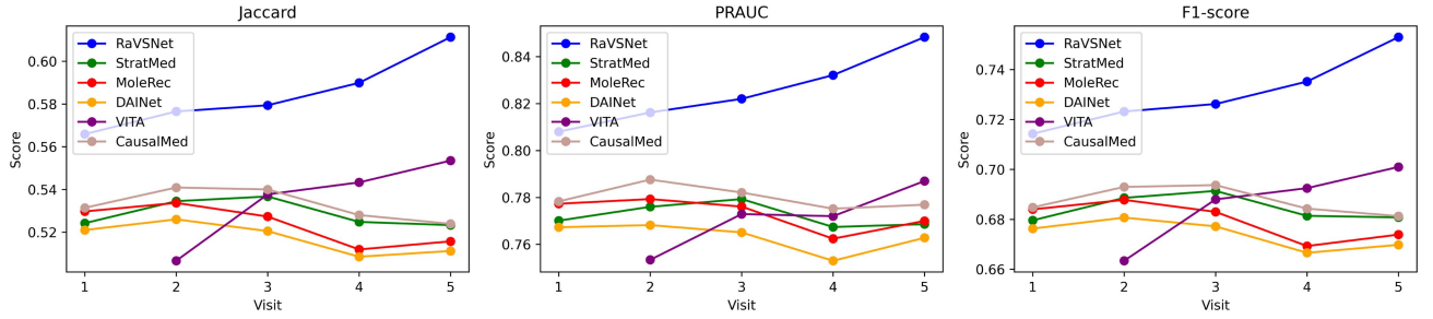
Fig. 4. Performance of different models across multiple visits.
