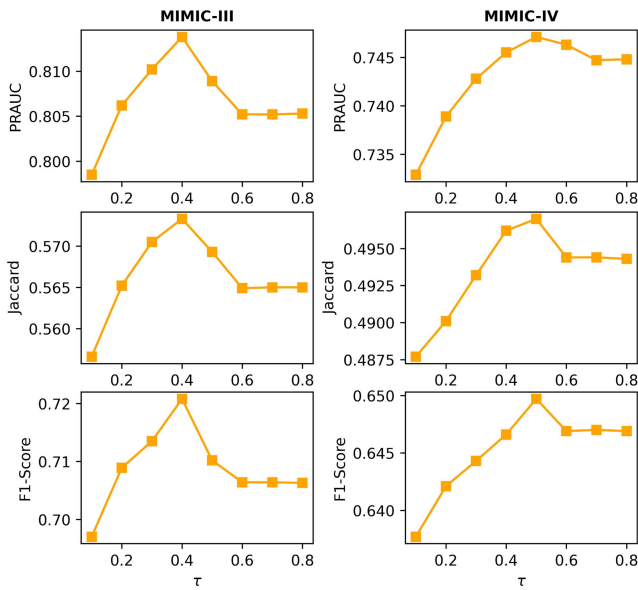
Fig. 6. Impact of \tau values on MIMIC-III and MIMIC-IV Dataset.
